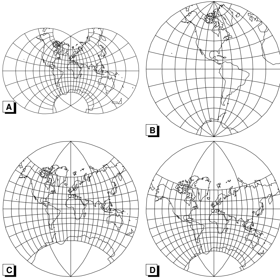
Figure 8.5: Lagrange Series
